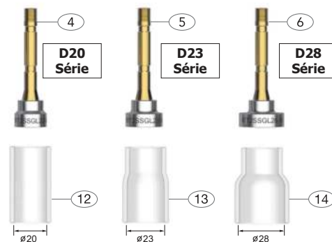
Hubice QUARTZ
